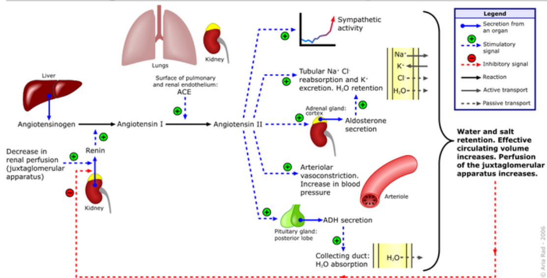
Figure 1: The renin-angiotensin-aldosterone pathway
